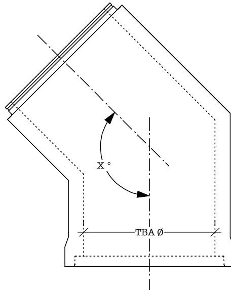
COUDE 750Ø @ 1800Ø X 2.5 M.LIN
